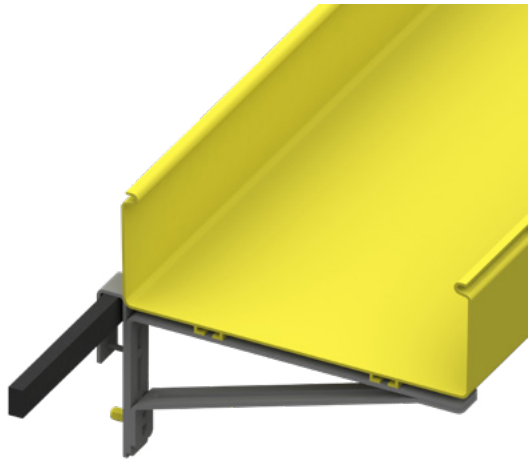
When using 200mm ducting with more than 25% cable fill and 300mm ducting with more than 20% cable fill the use of the strength bracket is recommended..
