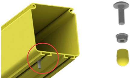
The duct features a slotted channel that accepts the coach bolt to provide a quick and easy mounting assembly.
